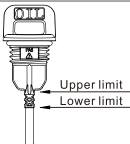
Oil level gauge
